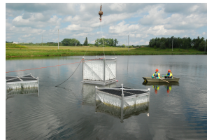
BioCord Lagoon Treatment and Geotube Sludge Management
